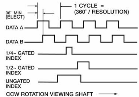
Figure 1 Output Waveforms
