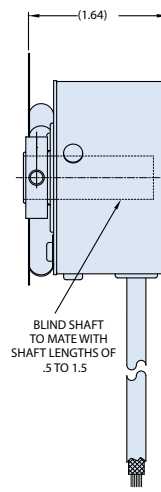
Blind Shaft
